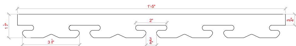
CM-BS-4-120 - 4 In Carrier
